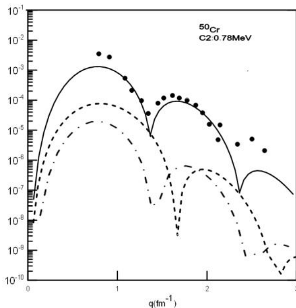
Figure(2): Inelastic longitudinal form factors for the transition to the 2+ in the ^{50}\text{Cr} with and without core-polarization effects and by using Tassie model, the experimental data are taken from Ref. [23]
