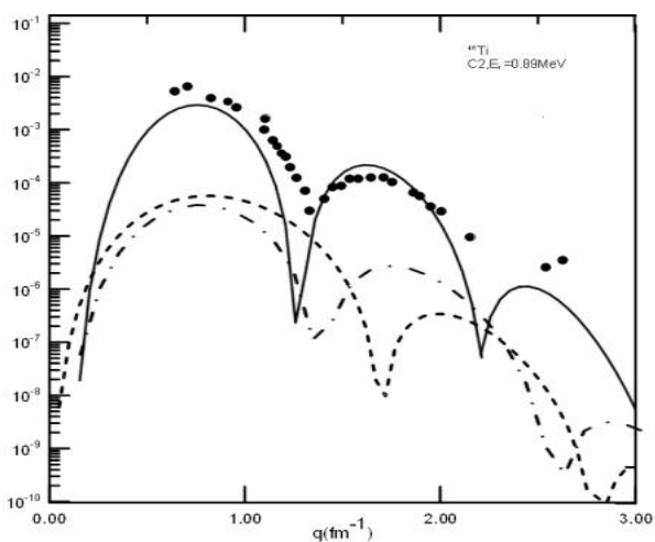
Figure(1): Inelastic longitudinal form factors for the transition to the 2+ in the ^{46}\text{Ti} with and without core-polarization effects and by using Tassie model , the experimental data are taken from Ref. [23]
