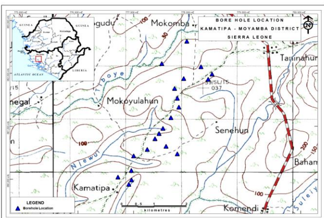
Figure1. Map of proposed mining site within the study area showing borehole locations
