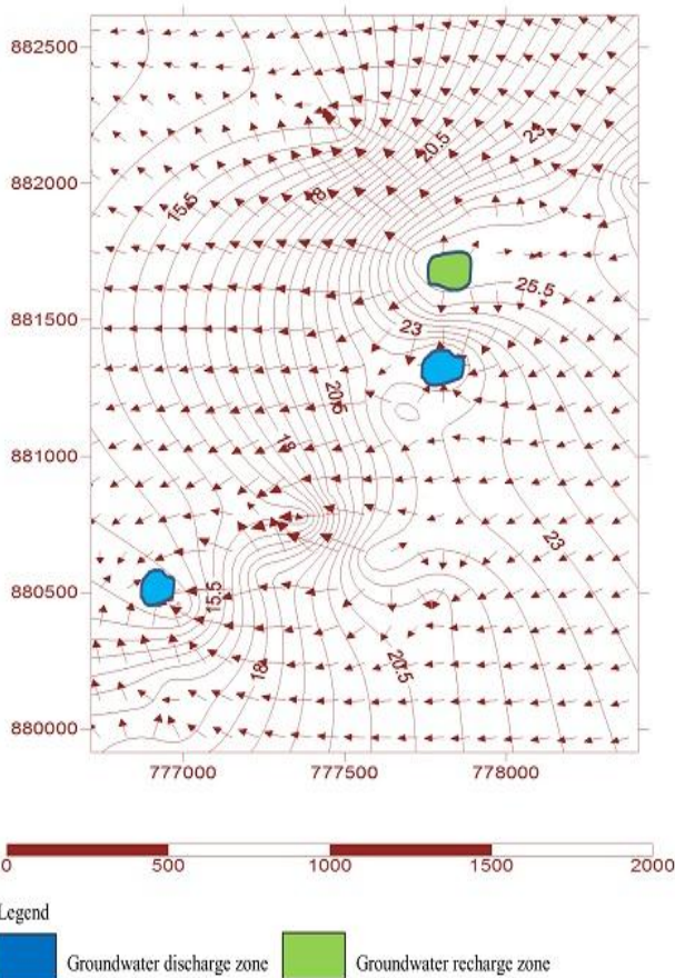
Figure5. A vector map superimposed on a water table contoured map of the study area. The figures represent hydraulic head values measured in meters. The arrows indicate flow directions. The blue patches depict groundwater discharge zones, while the green patch represents a zone of groundwater recharge.
