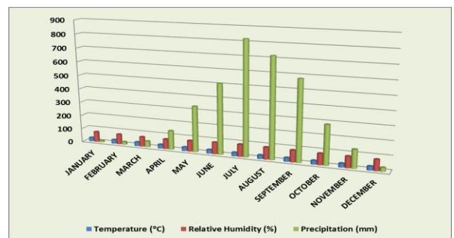
Figure2. Relationship between mean monthly temperature, relative humidity, and precipitation for the study area
