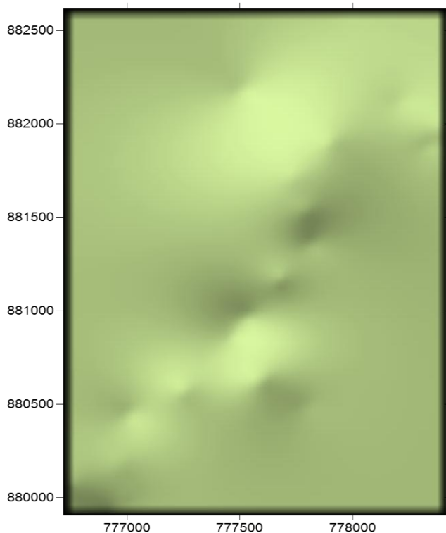
Figure6. Image map showing high points (recharge areas) and depressions (discharge areas).
